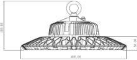
MAS-UFOH200A/MAS-UFOH240A
